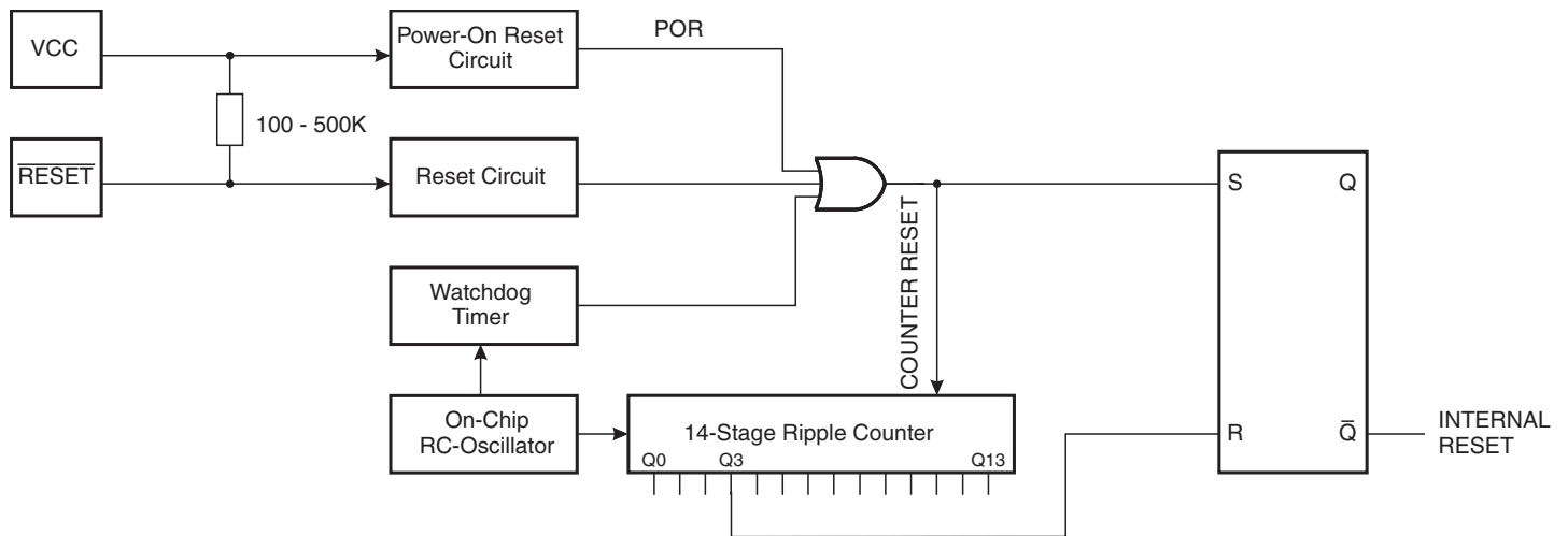
Figure 24. Reset Logic
