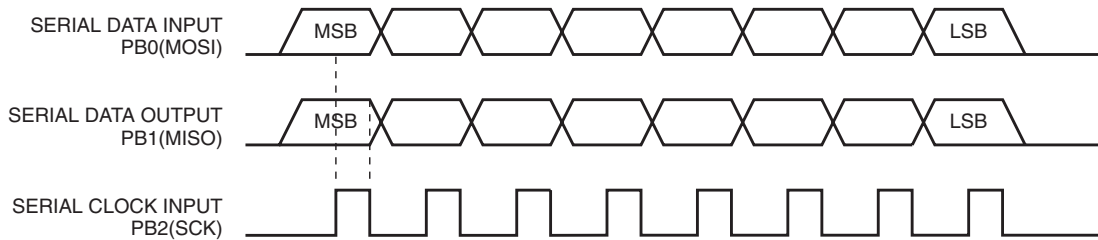
Figure 36. Low-voltage Serial Downloading Waveforms
